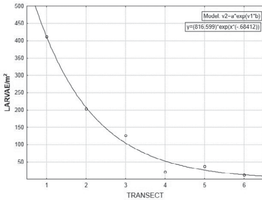
Fig. 6. Mean number of larvae per \text{m}^2 for all transects for Sep fitted with a significant P < 0.05 exponential curve where R = 0.993 .
