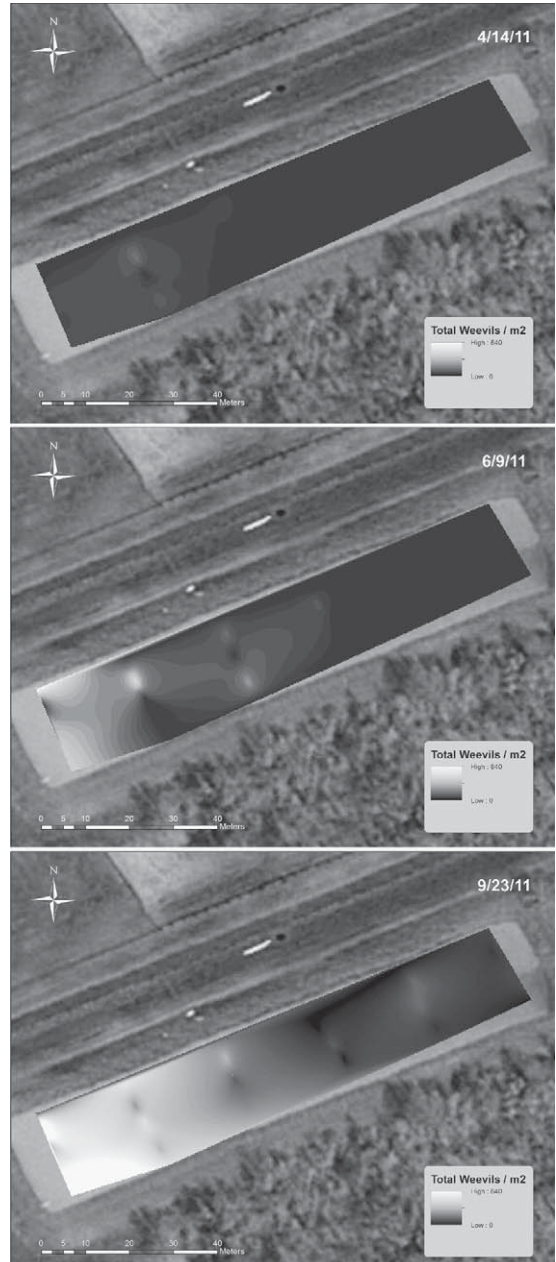
Fig. 7. Spatial analysis showing total weevil number per \text{m}^2 through time.
