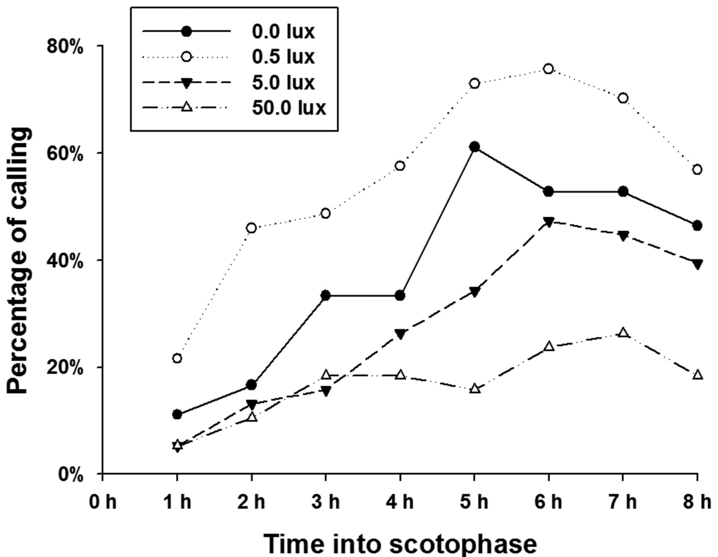
Fig. 1. Effects of light intensity and time into scotophase on percentage of virgin females calling. Thirty-seven to 40 female moths were used in each treatment. Percentage of calling = 100 \times number of calling females at the time point / total number of females.
