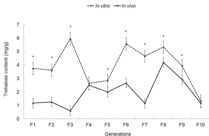
Fig. 3. Trehalose content in Trichogramma dendrolimi reared in vitro and in vivo for 10 generations. Means ( \pm SE) were calculated from 3 replicates. Data with an asterisk differ significantly according to paired-sample t -tests at P = 0.05 .
