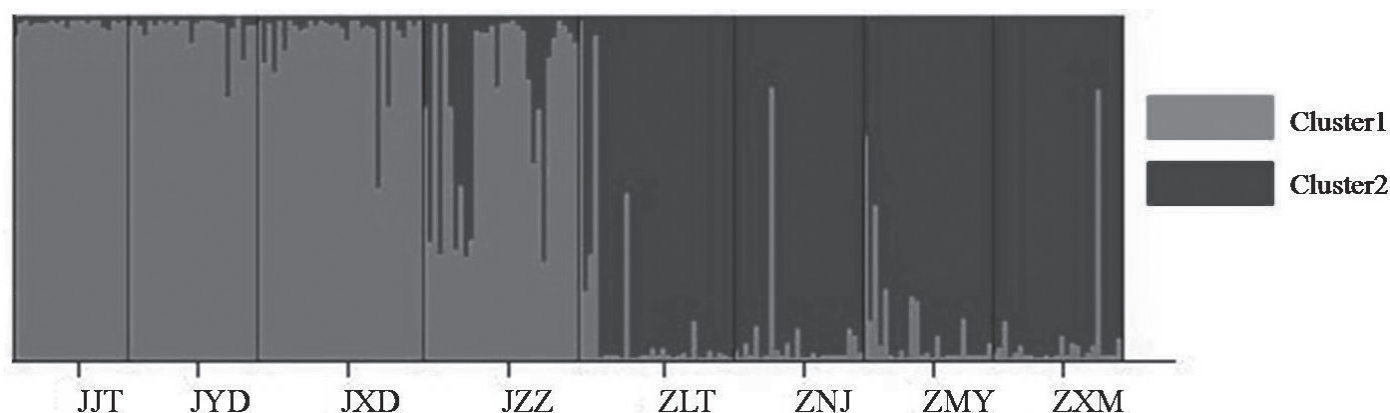
Fig. 2. Bayesian clustering analysis by use of STRUCTURE, which indicates the presence of 2 clusters. Proportion of membership coefficient for 8 Cydia pomonella populations falling into the 2 clusters is depicted by 2 different shades of gray, respectively. The sampling locations include JinTa (JJT), YinDa (JYD), XiDong (JXD) and ZongZai (JZZ) of Jiuquan Region, and Luo Tuo Cheng (ZLT), NiJiaying (ZNJ), MinYong (ZMY) and XiaoMan (ZXM) of Zhangye Region.
