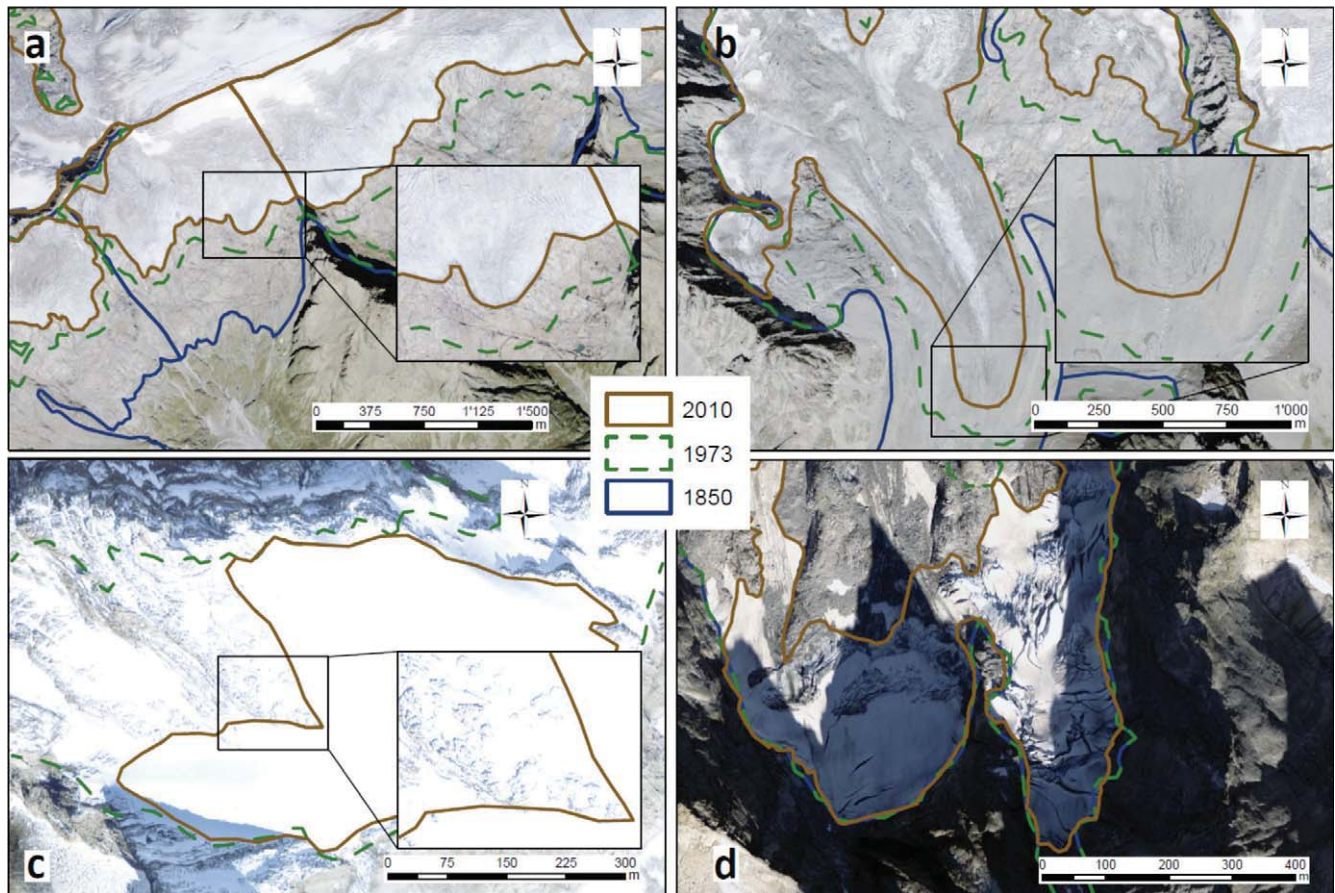
FIGURE 2. Examples of different situations encountered when mapping glacier outlines: (a) bare ice meets solid bedrock (Tellingletscher, 2011); (b) debris-covered marginal zones (Innre Baltschieder Gletscher, 2011); (c) snow-covered marginal zones (Bächistockfirn, 2010); and (d) shadowy areas (Vadrec da la Trubinasca-E, 2009). Digitized outlines from 1850 (navy blue), 1973 (dashed green), and 2010 (brown) are overlain to the respective SWISSIMAGE orthophoto tile based on which the latest outline was drawn.
