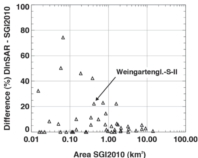
FIGURE 7. Relative difference between glacier outlines derived from combination of DInSAR interferograms and aerial orthophotos and glacier outlines derived from aerial orthophotos only versus glacier area 2010 for 48 individual glaciers in the Mischabel test region (Fig. 1).
