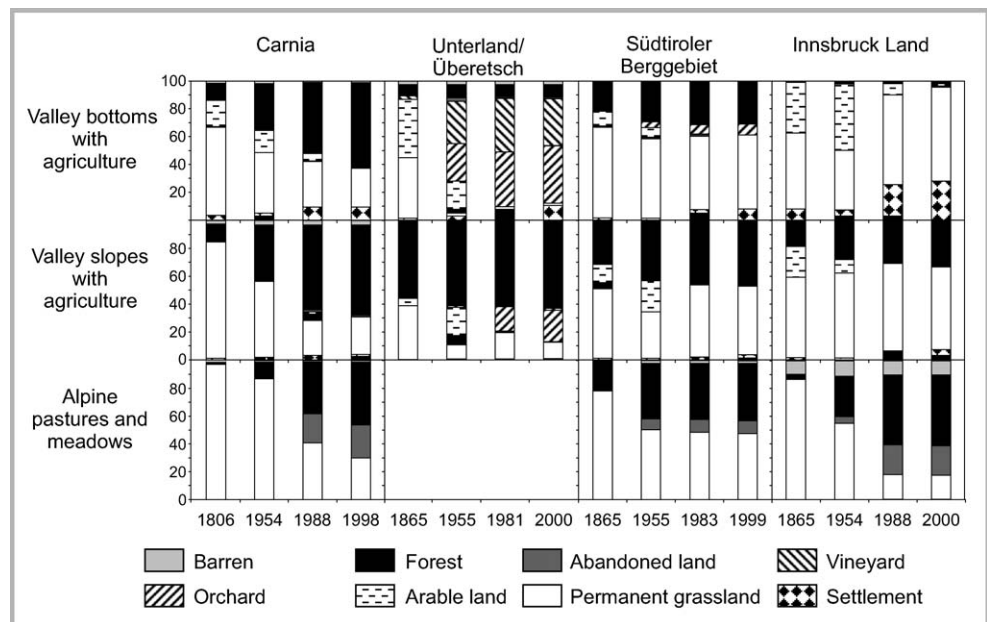
FIGURE 2 Historical land use development in 4 different agrarian regions of the European Alps: 1) the agricultural retraction region of Carnia (Italy), 2) the South-Tyrole wine and fruit cultivation region Unterland/Überetsch (Italy), 3) the South-Tyrole grassland region Südtiroler Berggebiet (Italy), and 4) the Innsbruck Land region (Austria). (Based on Tasser et al 2005)
