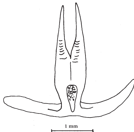
Fig. 6. Titillator of male E. jacquelineae (holotype) in posterior view.
