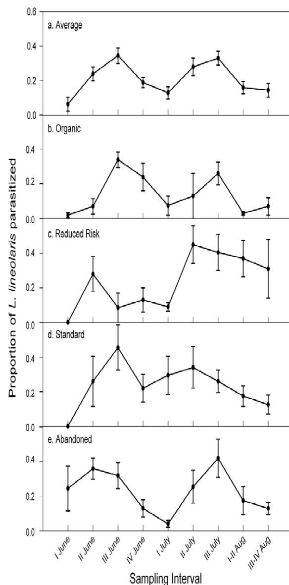
Figure 2. Mean parasitism, \pm standard error, of Lygus lineolaris by Peristenus spp. for a-all orchards combined; b- organic; c- reduced risk; d- standard; and e- abandoned orchards over time. All values represent data combined from 2005-2006. High quality figures are available online.
