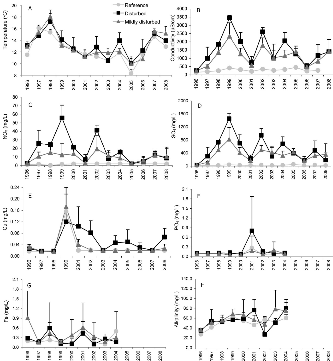
FIG. 2. Mean ( \pm 1 SD) winter temperature (A), conductivity (B), \text{NO}_3 (C), \text{SO}_4 (D), Cu (E), \text{PO}_4 (F), Fe (G), and alkalinity (H) of the water between 1996 and 2008.
