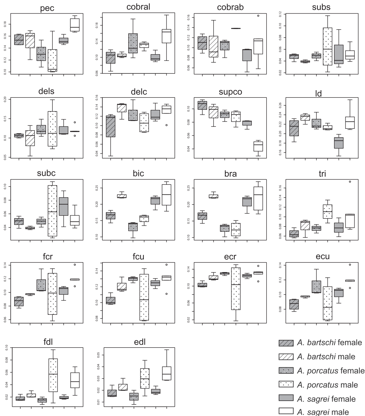
Fig. 4. Boxplots showing the normalized values for the forelimb muscles moment arm. The vertical axis indicates the ratios of the value to length of limb bone that the muscle inserts.
