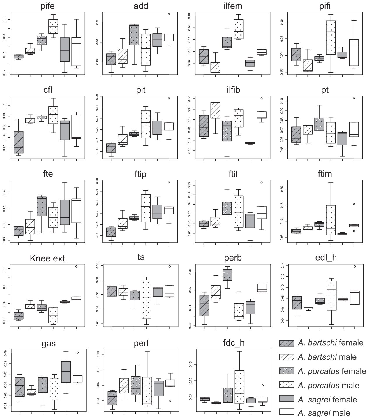
Fig. 5. Boxplots showing the normalized values for the hindlimb muscles moment arm. Result of four knee extensors ( M. iliobtibialis , M. ambiens , M. femorotibialis externus , M. femorotibialis internus ) are illustrated collectively in “Knee ext”, as these muscles insert to a common tendon.
