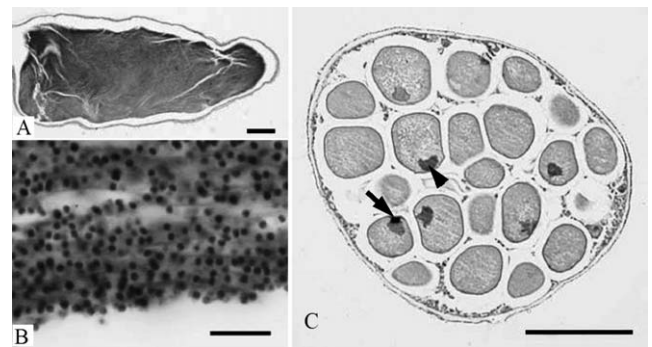
Fig. 3. Histological sections of the gonads of a male and the female of Coscinasterias acutispina 18 months after the completion of metamorphosis. (A) Testis from a long arm of individual Ca in Fig. 2. (B) Magnified view of testis in (A) black spheres are heads of sperm. (C) Ovary from a long arm of individual Baa in Fig. 2; arrowhead, germinal vesicle; arrow, nucleolus. Scale bars: A, C = 200 \mu m; B = 10 \mu m.
