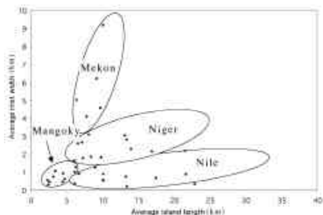
Figure 2. Plot of the average island length and average inlet width for all deltas. (A) Nile type islands plot near the X axis with the greatest island lengths and narrow ( < 1 km) inlets (Note: Magdalena and Ogooue Deltas not shown to reduce graph size. Average lengths and widths are 66 km/ 1.2 km and 43 km/ 1.1 km, respectively). (B) Niger type islands have somewhat shorter islands and inlet widths from 1 to 3 km. (C) Mangoky type islands plot along a similar trend as Niger type islands but have shorter island lengths (about 5 km) and inlets ( < 1 km). (D) Mekong type islands have inlets greater than 3 km and lengths from 5 to 10 km. Mississippi type islands are not grouped due to their variability, which is related to a distinct evolutionary stage of development.
