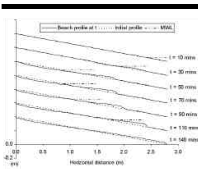
Figure 9. Time dependent beach profiles recorded from the tidal water depth experiment on a 1 in 7 beach under Condition II.
