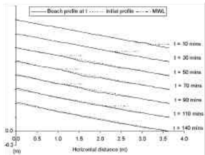
Figure 6. Time dependent beach profiles recorded from the tidal water depth experiment on a 1 in 9 beach under Condition II.
