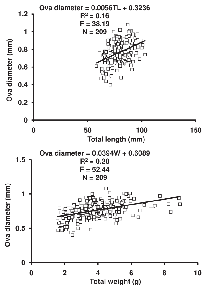
Fig. 6. Relationship between ova diameter and total length (mm) and total weight (g) of female Cobitis cf. satunini from the Siahroud stream, southern Caspian Sea (northern Iran).
