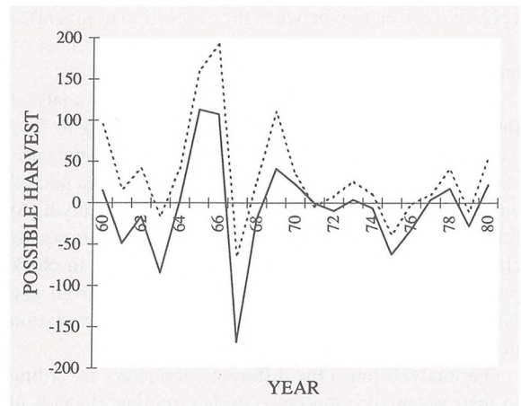
Figure 3. Number of willow grouse harvestable at Tranøy assuming mean adult apparent winter survival (0.51) and juvenile apparent winter survival (0.26), the yearly observed spring densities and year specific chick production (solid line). The dotted line represents the harvest if Myrberget (1988) underestimated apparent winter survival by 10% or willow grouse show a 100% compensation in natural survival rates for 10% increased mortality due to hunting. Negative values indicate that no harvest is possible and that the population declines regardless of hunting
