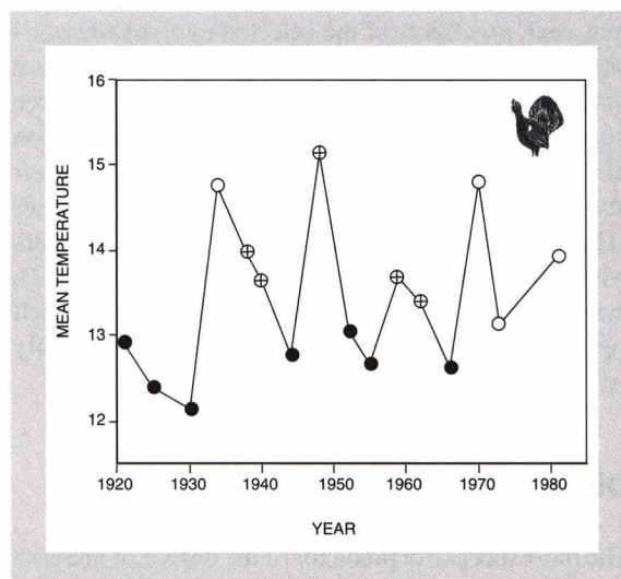
Figure 3. Mean temperature in June-September of the previous year for years with a bilberry production below average, but a production above average in the previous year (1/0 years). The years were further categorised based on the autumn population size of capercaillie, compared to the size in the previous year. ● symbolises years with a strong increase, ⊕ years with a slight increase, and ○ years with no increase in the capercaillie autumn population.
