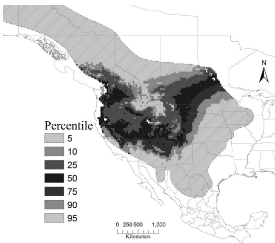
Figure 2. Isotopic basemap to naively estimate origins of Swainson's Hawks trapped in Butte Valley, CA, from 2008–2010. Estimates were based on feather \delta^2\text{H} values following Hobson et al. (2009) from feathers collected from known-source raptors. All feathers used in the analysis were growing at the time of capture and should reflect values from within the study area (white circle). Diagonal barring indicates breeding range of the Swainson's Hawk (Bechard et al. 2010).
