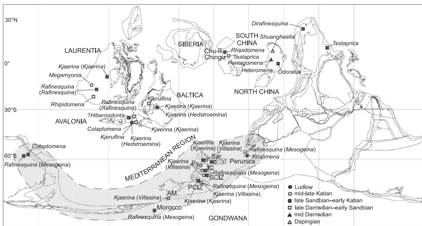
Fig. 20. First Appearance Datum (FAD) of all rafinesquinine genera in each palaeocontinent plotted over a palaeogeographical map for the late Katian time slice based on BugPlates and using a Mollweide projection. Present-day outlines of lands and seas are shown on each continent to aid recognition. AM, Armorican Massif; PCIZ, Portuguese Central Iberian Zone; SCIZ, Spanish Central Iberian Zone; IC, Iberian Chains; Py, Pyrenees; MN, Montagne Noire; Sar, Sardinia.
