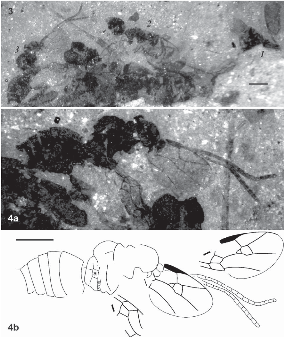
Figs 3, 4. Afropia variicornis sp. n.: (3) Paratypes BP/2/26666-3, 2 & 1, photograph; (4) Paratype BP/2/26666-3 & BP/2/28224-3, composite photograph and line drawing; a – areola. Scale bars = 1.0 mm.
