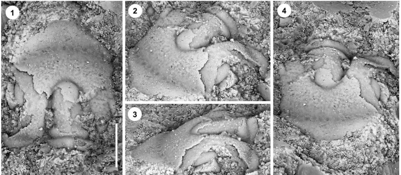
Figure 8. Oenonella sp. 2 from the Antelope Valley Formation (Dapingian), flanking beds of Meiklejohn bioherm, Meiklejohn Peak, Nye County, southern Nevada, USA. (1–4) Cranidium, NHM It 9810: (1) dorsal view; (2) oblique view; (3) left dorsolateral view; (4) anterodorsal view. Scale bar = 0.5 mm.
