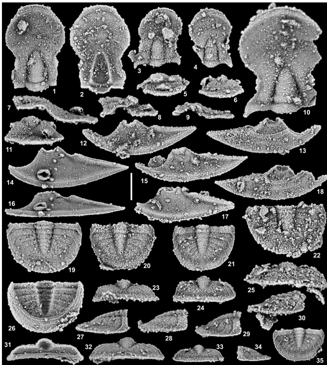
Figure 7. Oenonella otherfellersorum n. sp. from horizons TCM 2, TCM 13, and TCM 14*, Table Cove Formation (Darrivillan), near Marechal Island, Hare Bay, western Newfoundland, Canada. (1, 2, 7, 11) Cranidium, holotype, GSC 142613: (1) dorsal view; (2) ventral view; (7) right lateral view; (11) anterior view (TCM 14*). (3, 5, 8) Cranidium, GSC 142614: (3) dorsal view; (5) anterior view; (8) right lateral view (TCM 14*). (4, 6, 9) Cranidium, GSC 142615: (4) dorsal view; (6) anterior view; (9) right lateral view (TCM 13). (10) Cranidium, GSC 142616, dorsal view (TCM 13). (12, 13) Left librigena, GSC 142617: (12) external view; (13) internal view (TCM 14*). (14, 16) Left librigena, GSC 142618: (14) external view; (16) lateral view (TCM 13). (15, 18) Left librigena, GSC 142619: (15) external view; (18) internal view (TCM 14*). (17) Left librigena, GSC 142620, external view (TCM 14*). (19, 26, 27, 31, 32) Pygidium, GSC 142621: (19) dorsal view; (26) ventral view; (27) right lateral view; (31) anterior view; (32) posterior view (TCM 13). (20, 23, 28) Pygidium, GSC 142622: (20) dorsal view; (23) posterior view; (28) right lateral view (TCM 2). (21, 24, 29) Pygidium, GSC 142623: (21) dorsal view; (24) posterior view; (29) right lateral view (TCM 13). (22, 25, 30) Pygidium, GSC 142624: (22) dorsal view; (25) posterior view; (30) right lateral view (TCM 14*). (33–35) Pygidium, GSC 142625: (33) posterior view; (34) left lateral view; (35) dorsal view (TCM 13). Scale bar = 0.5 mm.
