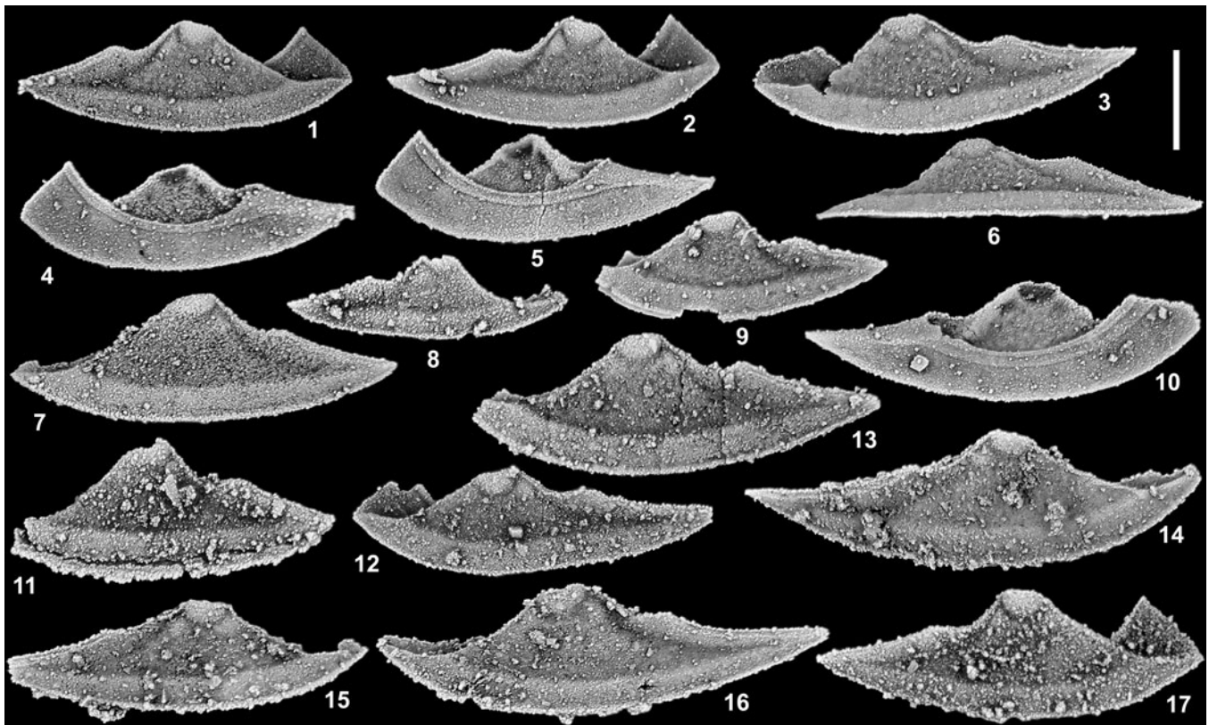
Figure 5. Oenonella wasisnamei n. sp. from horizons TCM 2, TCM 13, and TCM 18, Table Cove Formation (Darriwilian), near Marechal Island, Hare Bay, western Newfoundland, Canada. (1, 4) Right librigena, GSC 142590: (1) external view; (4) internal view (TCM 2). (2, 5) Right librigena, GSC 142591: (2) external view; (5) internal view (TCM 2). (3, 6, 10) Left librigena, GSC 142592: (3) external view; (6) lateral view; (10) internal view (TCM 18). (7) Left librigena, GSC 142593, external view (TCM 2). (8) Right librigena, GSC 142594, external view (TCM 13). (9) Left librigena, GSC 142595, external view (TCM 2). (11) Left librigena, GSC 142596, external view (TCM 13). (12) Left librigena, GSC 142597, external view (TCM 18). (13) Left librigena, GSC 142598, external view (TCM 2). (14) Right librigena, GSC 142599, external view (TCM 18). (15) Right librigena, GSC 142600, external view (TCM 18). (16) Left librigena, GSC 142601, external view (TCM 18). (17) Right librigena, GSC 142602, external view (TCM 2). Scale bar = 0.5 mm.
