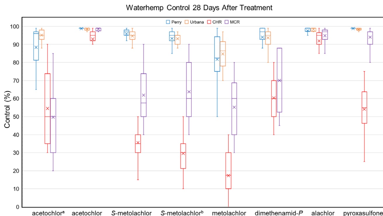
Figure 1. Waterhemp control at each location with eight different very-long-chain fatty acid (VLCFA)-inhibiting herbicides at 28 d after treatment. Blue, orange, red, and purple boxplots correspond to the Perry, Urbana, CHR, and MCR locations, respectively. a Encapsulated formulation. b Contains the herbicide safener benoxacor.
