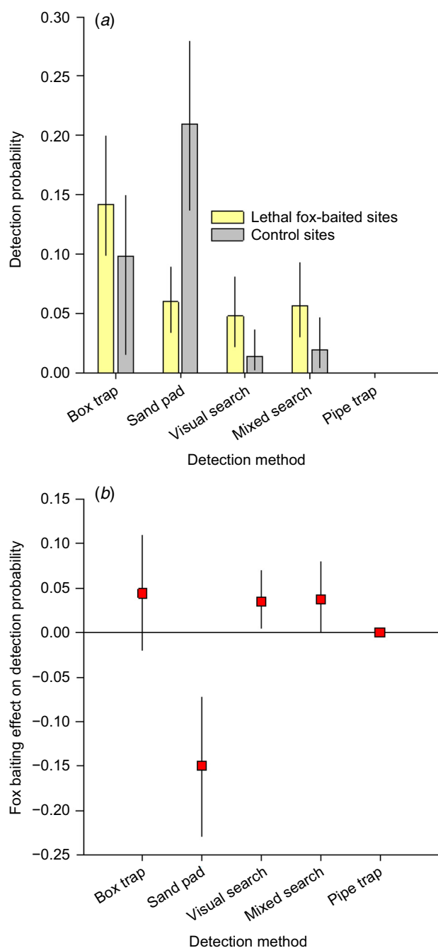
Fig. 3. (a) Method-specific lace monitor detection probabilities estimated for lethal fox baited or control (i.e. non-lethal fox-baited) sites. (b) The effect sizes of fox baiting on method-specific detection probability. All estimates report the posterior mean and 95% credible intervals.
