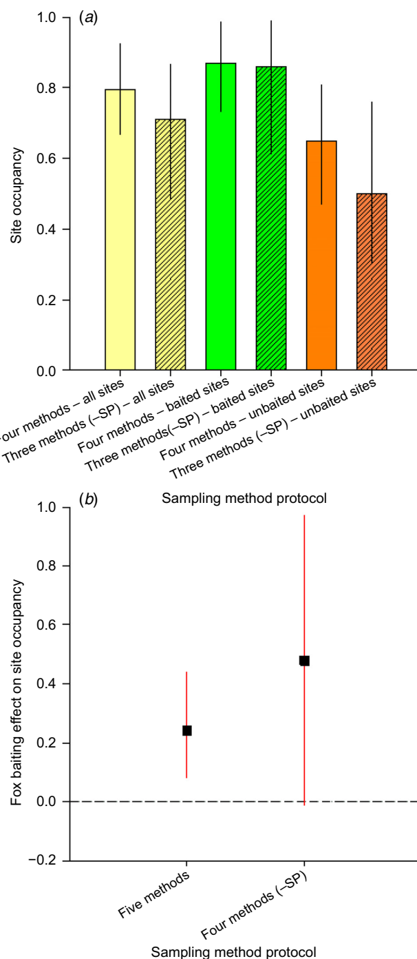
Fig. 4. (a) Multi-method site occupancy estimates of lace monitors for the entire study area and at fox-baited and unbaited (i.e. control) sites. Bars with hatching indicate the site occupancy estimates in which detection data from sand pads (i.e. SP) has been excluded. (b) The effect sizes of fox baiting on lace monitor site occupancy under the full method monitoring design and where detection data from sand pads have been excluded (i.e. drop SP). All estimates report the posterior mean and 95% credible intervals.
