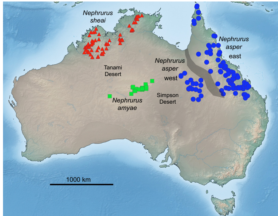
Fig. 1. Distribution of recognised taxa in the Nephurus asper group based on museum voucher specimens: Nephurus sheai (red triangles), N. amya (green squares) and N. asper (blue circles). Large areas of vertisol soils with largely treeless grassland ‘the Mitchell Grass Downs’ that separate Queensland records of N. asper into east and west distributional blocks are also indicated with grey shading.
