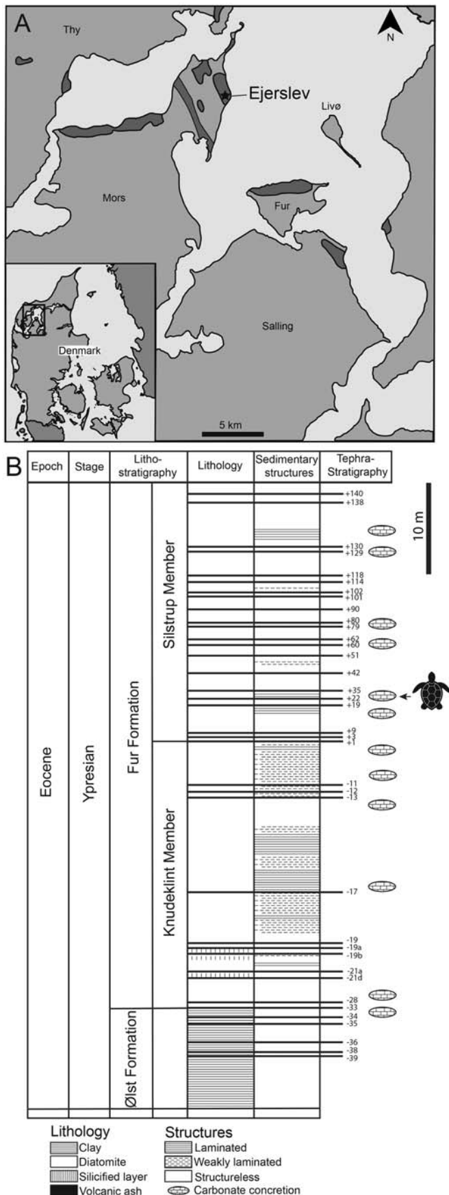
FIGURE 1. A , map of the Limfjord region of northern Jutland, Denmark, showing the geographic extension of Fur Formation strata (depicted in dark gray) and the approximate location of the Ejerslev Quarry in which DK 807 was found. Modified from Pederson and Buchardt (1996:fig. 1). B , stratigraphic column of the upper Ølst Formation and Fur Formation with the approximate horizon yielding DK 807 indicated by a sea turtle silhouette. Modified from Rasmussen et al. (2016:fig. 5).
