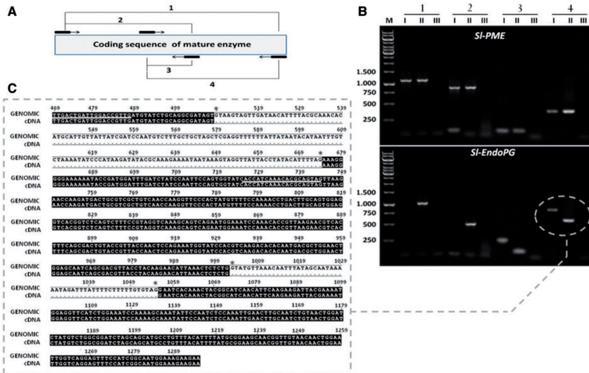
Fig. 4. Pectinase fragments amplified from S. levis cDNA and genomic DNA. PCR conducted with primers used for cloning ORFs in pPICZα vectors and primers for qRT-PCR analysis. (A) Representative scheme of primer position on coding sequence of mature SI-pectinases. (B) Gel separation of fragments generated by PCR; M, GeneRuler ladder 1 kb (Thermo Scientific Fermentas, CA); 1–4, primer combinations; I, reaction with genomic DNA template; II, reaction with cDNA template; III, negative control. (C) Alignment between SI-endoPG sequences from both genomic and cDNA samples, showing two small introns. Sequences underlined in white indicate forward and reverse primers used for sequencing of genomic SI-endoPG. Asterisks indicate 5' and 3' of two introns identified.
