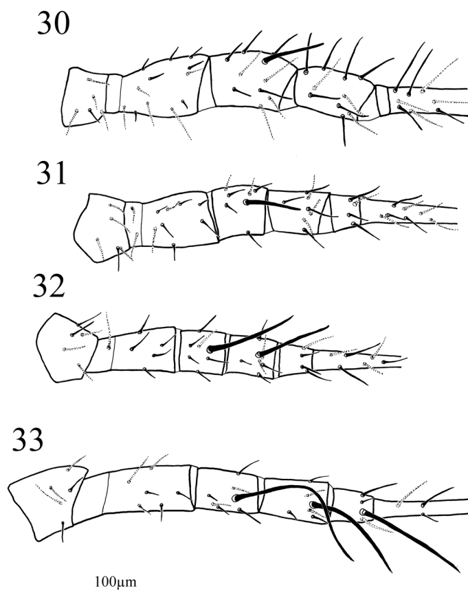
FIGURES 30–33. Amblyseius cinctus Corpuz & Rimano, 1966, female, legs (trochanter–basitarsus). 30. Leg I; 31. Leg II; 32. Leg III; 33. Leg IV.
