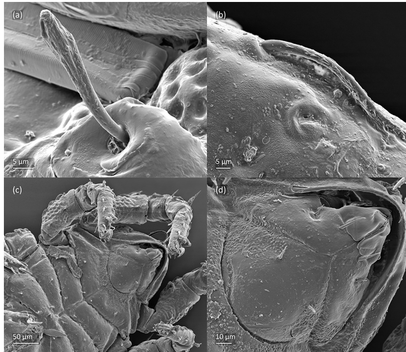
FIGURE 7. Platynothrus troendelagicus A. et S. Seniczak sp. nov. , adult, SEM micrographs. Bothridium and bothridial seta, dorsal view; (b) opisthonotal gla opening, dorsal view; (c), (d) anterior part, ventral view.
