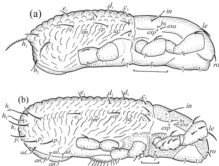
FIGURE 13. Platynothrus troendelagicus A. et S. Seniczak sp. nov. , lateral aspect, legs partially drawn, scale bars 20 \mu m. (a) Larva, (b) tritonymph.
