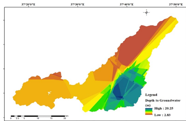
Figure 6. Groundwater depth map of Jedeb watershed.
