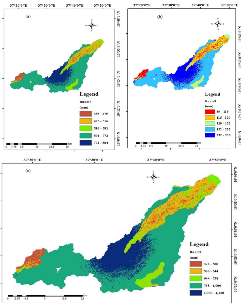
Figure 9. (a) Summer, (b) winter, and (c) annual simulated runoff of Jedeb watershed.
