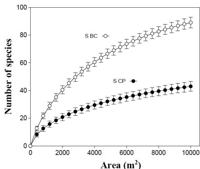
Figure 1. Species-area accumulation curve for CP and a typical one-hectare plot from BCI.
