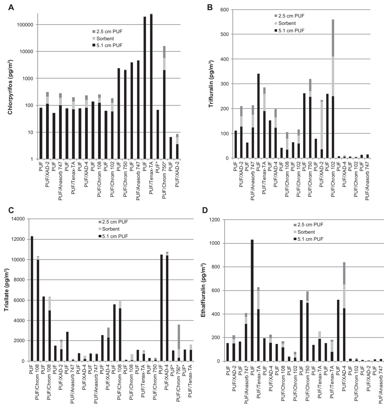
Figure 1. Atmospheric concentration of pesticides obtained from two co-located PS-1 samplers for sampling periods where pesticides reached sorbent layer. Pesticides: A ) chlorpyrifos; B ) trifluralin; C ) triallate; D ) ethalfluralin. PUF refers to PS-1 sampler containing 7.6 cm PUF, and PUF/Sorbent refers to PS-1 sampler containing 5.1 cm PUF/14 g sorbent/2.5 cm PUF with sorbent specified.
