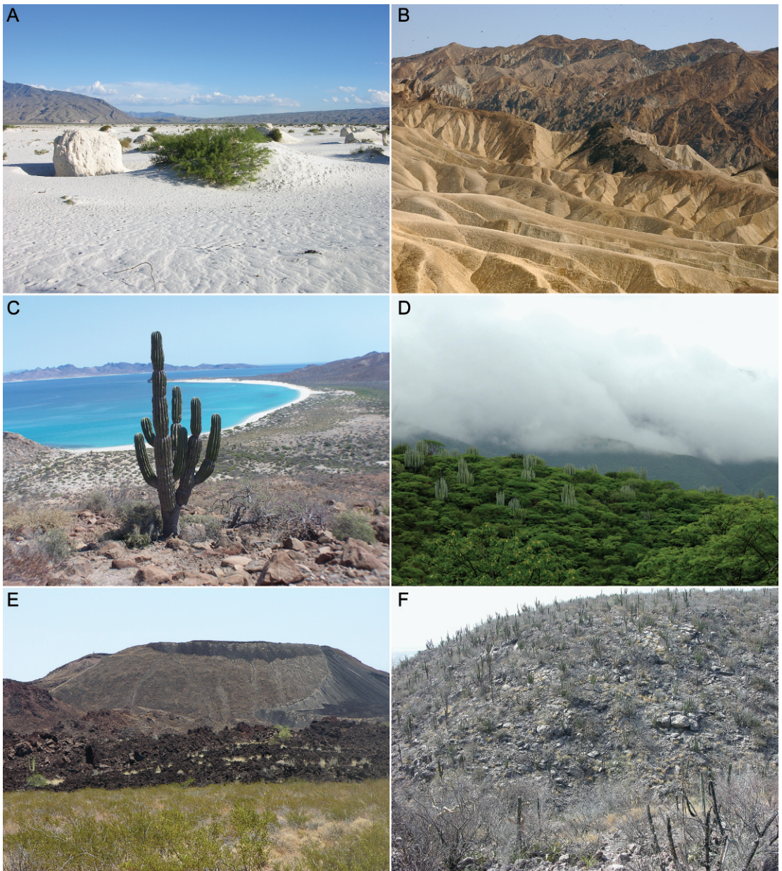
Fig. 2. Representative habitats of species in the North American vaejovoid scorpion subfamily Syntropinae Kraepelin, 1905. A. Cuatro Ciénegas de Carranza, Coahuila, Mexico, habitat of Chihuahuanus cazieri (Williams, 1968), comb. nov., Chihuahuanus coahuilae (Williams, 1968), comb. nov., and Chihuahuanus globosus (Borelli, 1915), comb. nov. B. Death Valley, California, habitat of Kochius hirsuticauda (Banks, 1910). C. Isla Espiritu Santo, La Paz, Baja California Sur, Mexico, habitat of Kochius insularis (Williams, 1971), Paravaejovis diazi (Williams, 1970), comb. nov., and Paravaejovis gravicaudus (Williams, 1970), comb. nov. D. Cuicatlán, Oaxaca, Mexico, habitat of Mesomexovis subcristatus (Pocock, 1898), comb. nov. E. Pinacate desert, Sonora, Mexico, habitat of Paravaejovis confusus (Stahnke, 1940), comb. nov. F. West of La Paz, Baja California Sur, Mexico, habitat of Syntropis williamsi Sologlad et al., 2007. Photos in B and E courtesy of R. Mercurio and in C courtesy of I.G. Nieto.
