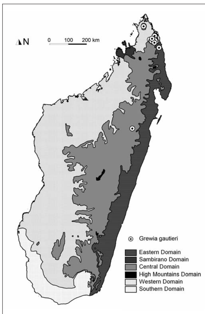
Fig. 4. – Map showing the distribution of Grewia gautieri Wahlenst & Nusb. in Madagascar (circles), plotted on the map of phytogeographical domains sensu HUMBERT (1955).
