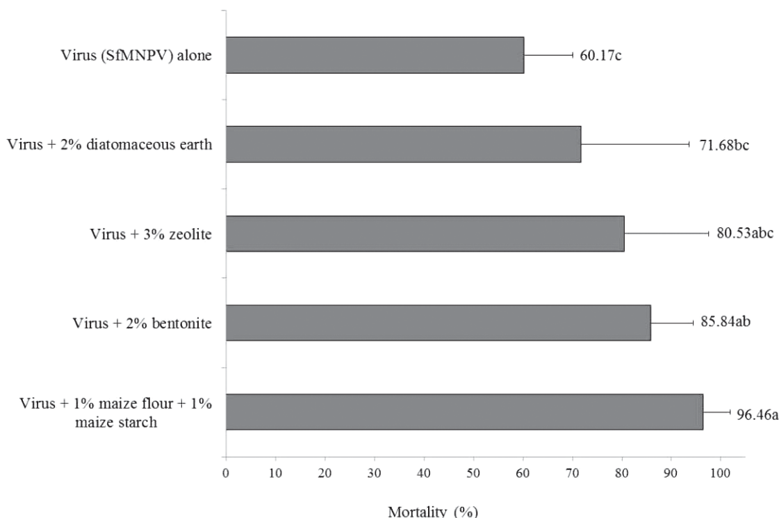
Fig. 1. Mortality rates of Spodoptera frugiperda when first instars were fed on maize plantlets treated with SfMNPV occlusion bodies (OBs) alone or as formulations (wettable powder) amended with a thickening agent (xanthan gum at 0.5%) and an adjuvant (Pegodel™ at 1%, Syngenta). Error bars indicate standard deviation from the mean of mortality responses observed among replicates. The value beside each error bar indicates the percent mortality, and letters indicate significant differences compared with the control and treatments involving virus OBs alone according to Tukey's test ( P > 0.05 ). Concentrations of test substances are given as percentage wt/wt.
