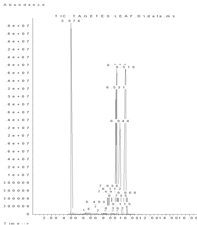
Fig. 2. Total ion current (TIC) mode chromatographic plot of marigold leaf volatiles sampled using the thermal desorption (TD) technique.
