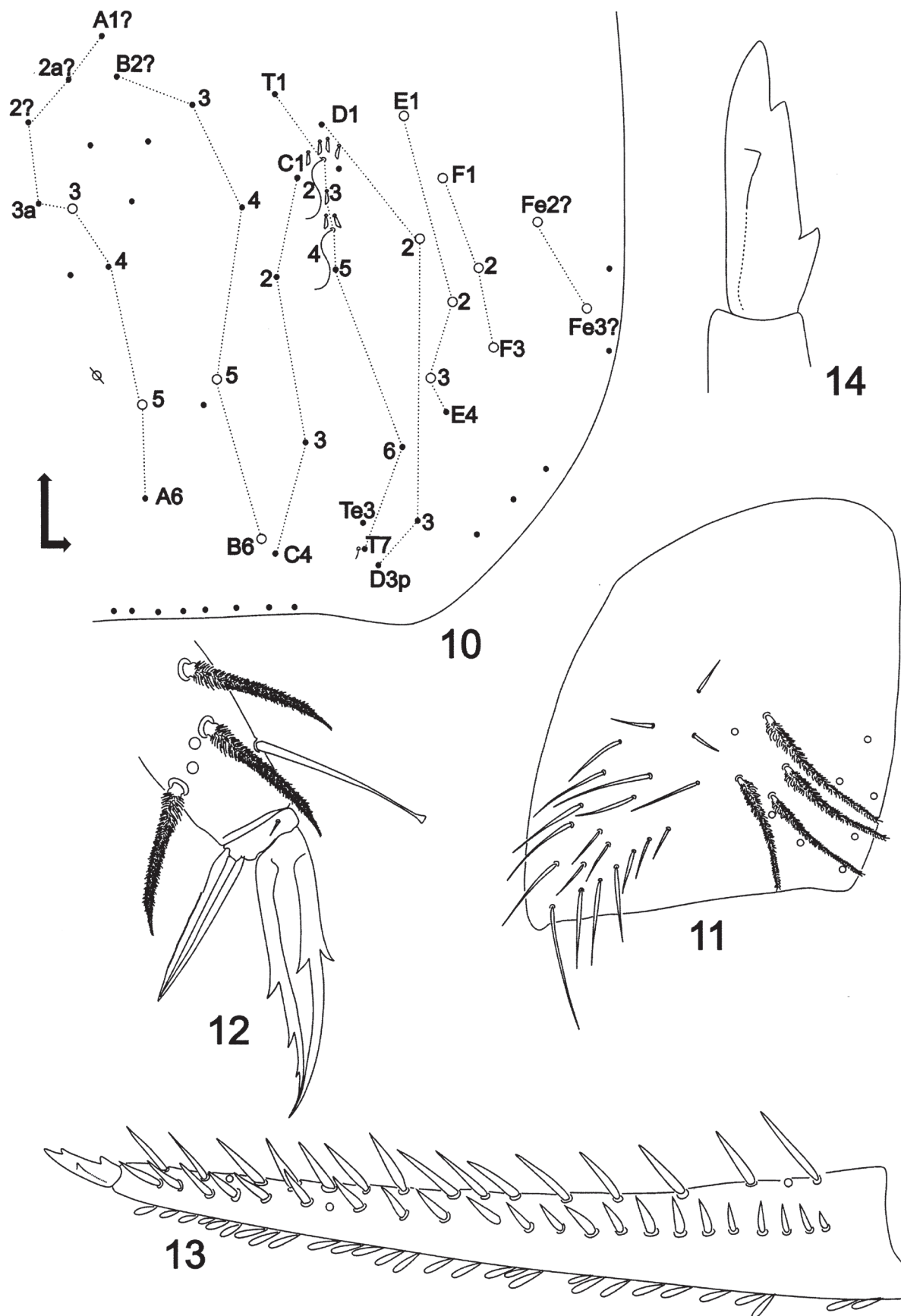
Figs. 10-14. Lepidonella zeppelinii sp. nov.; (10) Dorsal chaetotaxy of abdomen 4; (11) Trochanteral organ; (12) Metathoracic claw complex; (13) Dens and mucro; (14) Detail of mucro.
