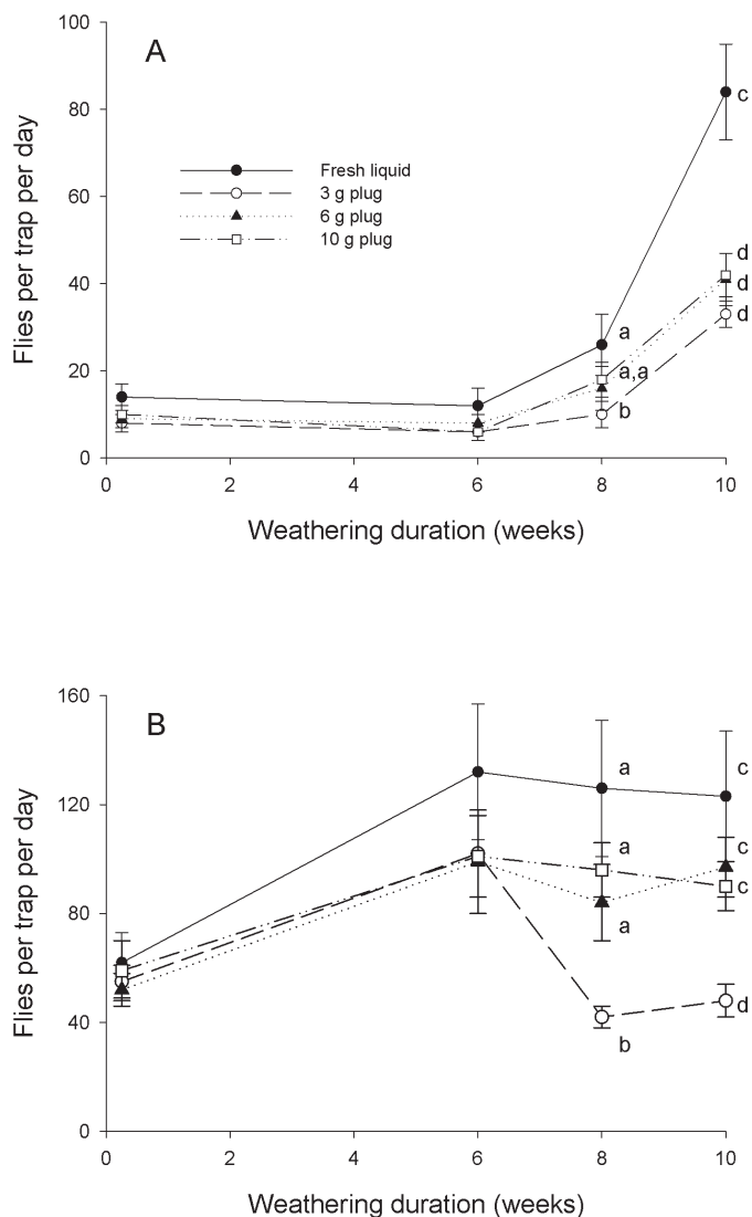
Fig. 2. Captures of Bactrocera dorsalis males on Oahu, Hawaii, USA, in Jackson traps baited with fresh liquid methyl eugenol or weathered, polymeric plugs containing 3, 6, or 10 g of methyl eugenol, where accompanying dichlorvos squares were either weathered (A, Experiment 2) or replaced prior to each trapping period (B, Experiment 3). Symbols represent means \pm 1 SE; n = 12 in all cases. For a given trapping interval, means marked with different letters differed significantly ( P < 0.05 , Tukey test).
