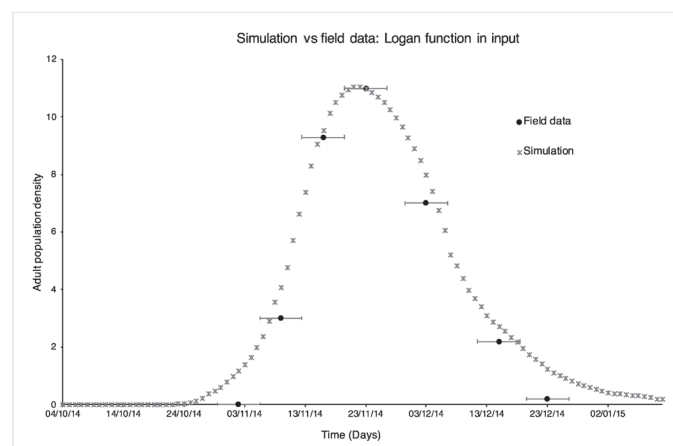
Fig. 2. Simulation output from the model (1) evaluating the daily average temperature with the Logan development rate function.
