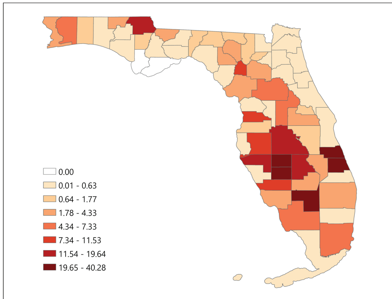
Fig. 2. Heat map showing the relative contribution of insect pollinators to agriculture in each county in Florida. Values were calculated as acreage per crop per county*average pollinator contribution value per crop (proportion 0–1), summed across all plant-based crops in each county and divided by the county's total area.
