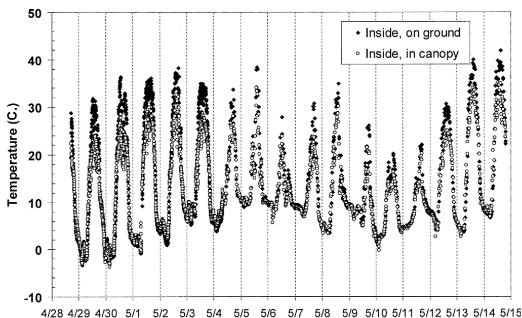
Fig. 3. Surrogate temperatures inside cages on the ground and at canopy level during the course of the immature Mormon cricket observation period. Symbols: ♦ "Inside, on ground" thermal surrogate positioned on the bare ground simulating basking insect; ○ "Inside, in canopy" thermal surrogate positioned on a bamboo skewer 10cm above the ground, simulating Mormon cricket roosting in plant canopy.
