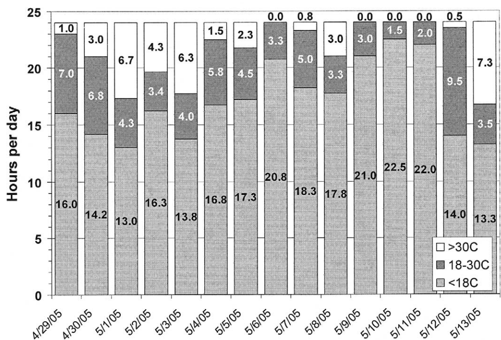
Fig. 5. Daily accumulated hours of temperatures optimal and sub-optimal for fungal growth, based on thermal surrogates inside cages and on the ground.
