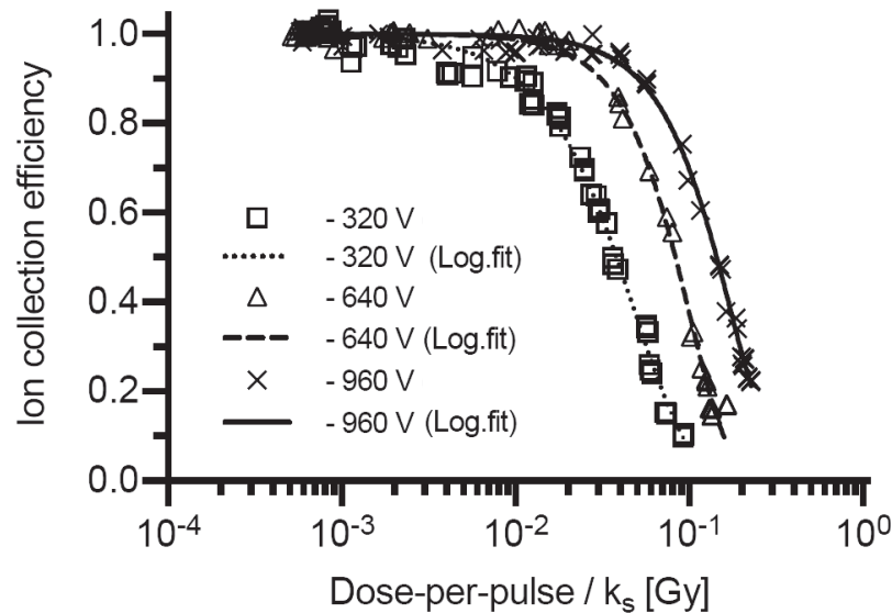
FIG. 5. Ion-collection efficiency of the transmission chamber as a function of DPP/k_s , according to simultaneous chamber and film measurements, for negative polarizing voltages of 320 V, 640 V and 960 V, together with a logistic function (Eq. 12) fitted to the data points.
