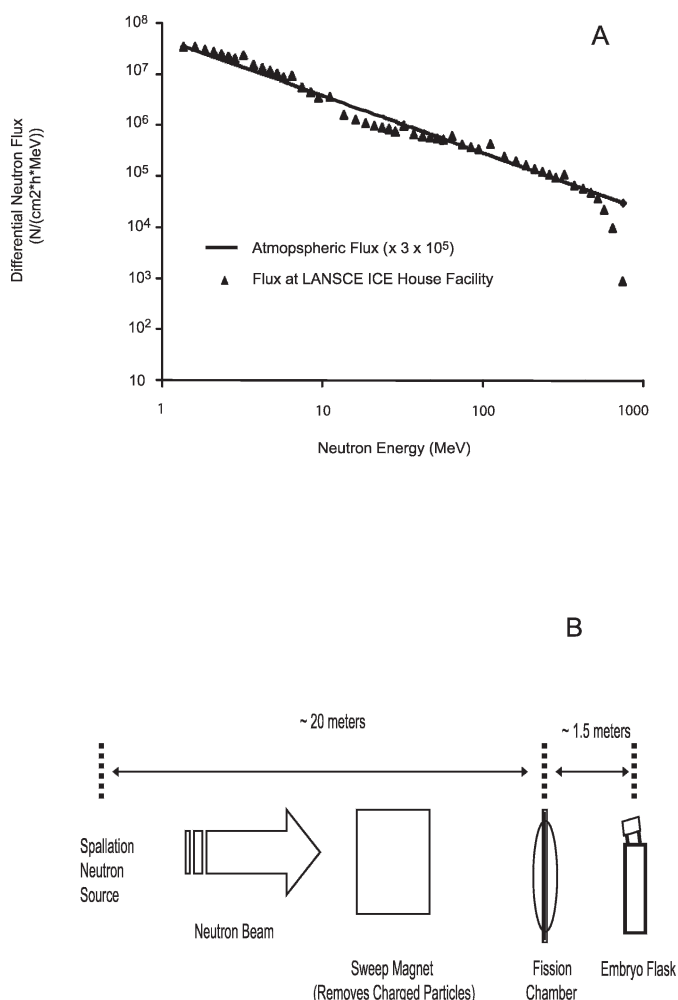
FIG. 1. Panel A: Differential energy spectrum of the LANSCE/WNR neutron beam line used in this study, and neutron flux found at an altitude of 12,000 m in the atmosphere. Panel B: Medaka irradiation using the 30L LANSCE/WNR neutron beam line. Relative positions of the neutron source, sweep magnet, fission chamber and embryo flask are shown (figure is not to scale). In some experiments, a TEPC was placed in line behind the embryo flask for dosimetry purposes.
