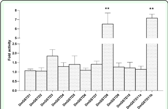
Figure 1. Delta class glutathione transferases (DmGSTs) modulate p38b kinase activity toward the substrate ATF2 in Drosophila melanogaster . The histogram shows changes in fold activity the DmGSTs have on p38b phosphorylation rates compared to the reaction without DmGSTs. The experiments were performed in triplicate. One-way ANOVA with Dunnett's multiple comparison test was performed with kinase reaction lacking DmGST as a control; statistical significance is shown by ** for p <0.01. High quality figures are available online.
