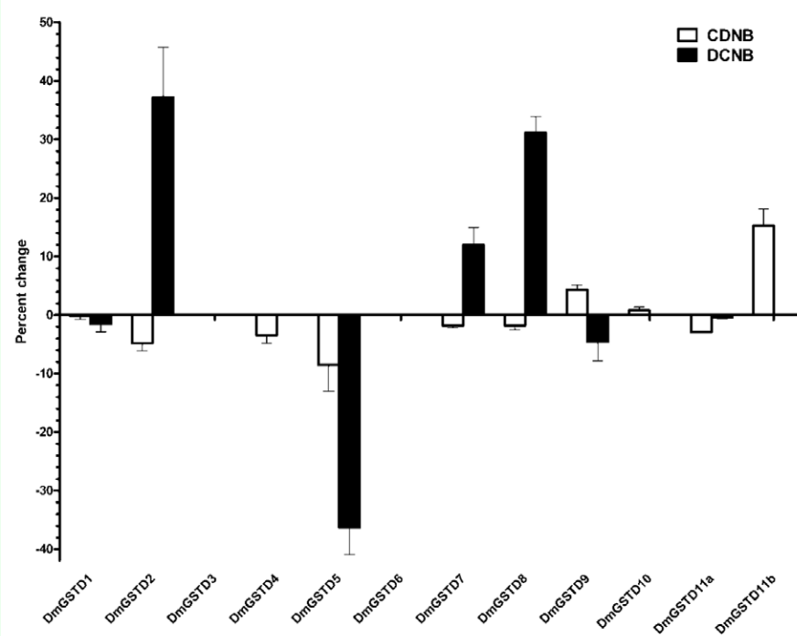
Figure 3. p38b changes the substrate specificities of Delta class glutathione transferases (DmGSTs) in Drosophila melanogaster . DMGSTs and p38b were incubated in 1:1 molar ratio for five minutes at room temperature. DmGST activity was measured using CDNB and DCNB as substrates. The percentage change in DmGST activity was calculated by comparing the reactions in the presence and absence of p38b. Results shown are representative of triplicate independent experiments. High quality figures are available online.
