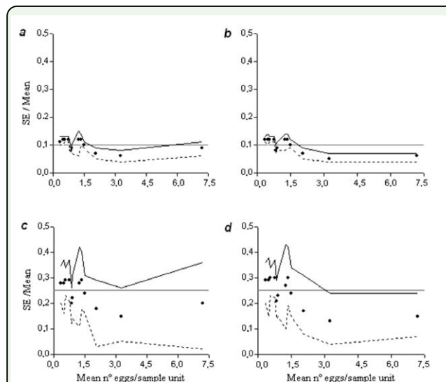
Figure 4. Summary of resampling validation analysis using 12 independent data sets of Colias lesbia eggs on alfalfa showing the average precision levels ( C = \text{SE}/\text{Mean} ) for Green's sequential sampling plan (graphs a and c) and for Kuno's sequential sampling plan (graphs b and d). Precision levels for the sampling plans were: C = 0.10 (graphs a and b) and C = 0.25 (graphs c and d). Horizontal lines in a and b represent the desired precision level of 0.10, and horizontal lines in c and d represent the desired precision level of 0.25. Black circles denote mean values; solid lines and dashed lines denote the maximum and minimum values, respectively. High quality figures are available online.
