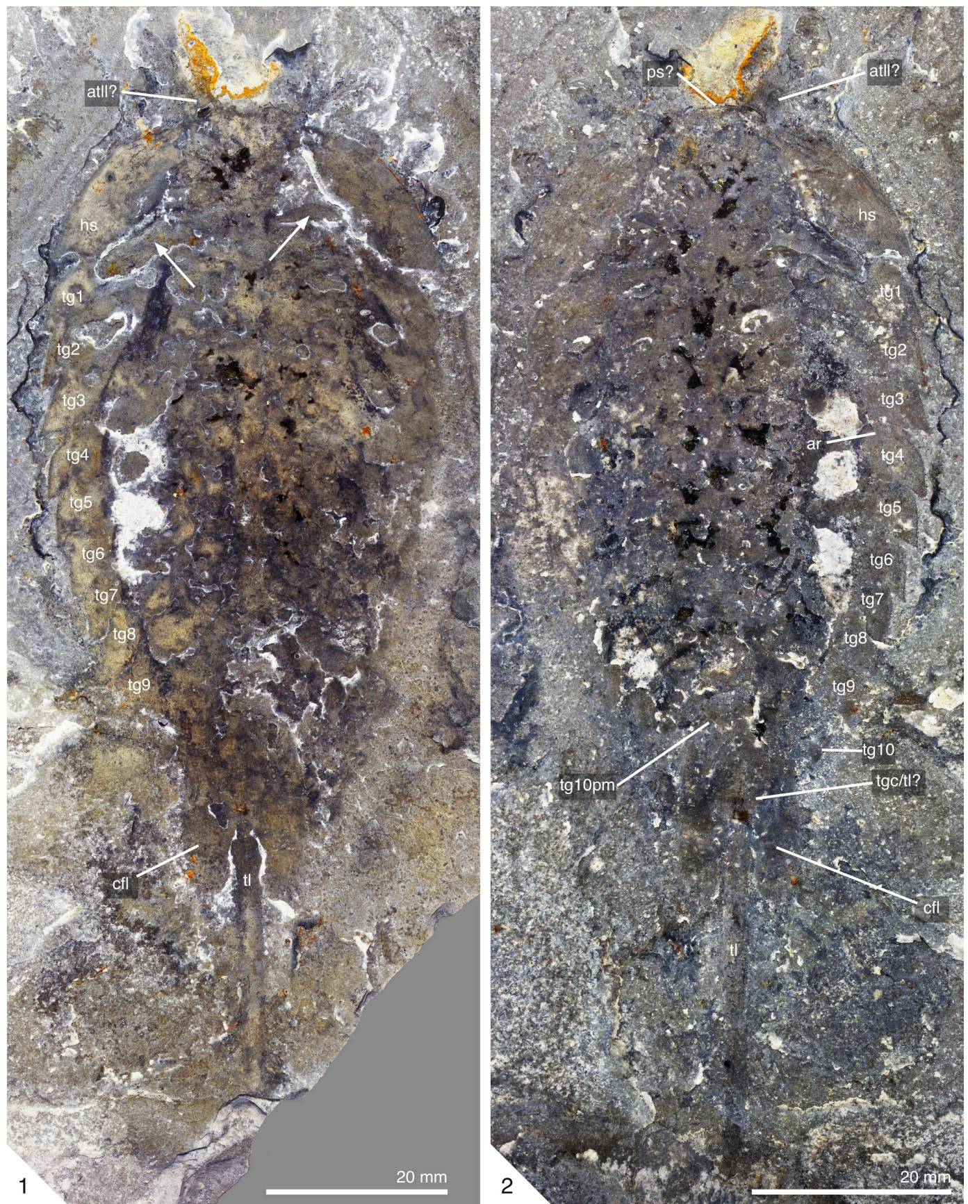
Figure 1. Emeraldella brutoni n. sp., KUMIP 321500, immersed in alcohol, using crossed polarizers. 1, Part, overview of specimen, arrows indicate possible remnants of limbs; 2, counterpart, overview of specimen (new).
