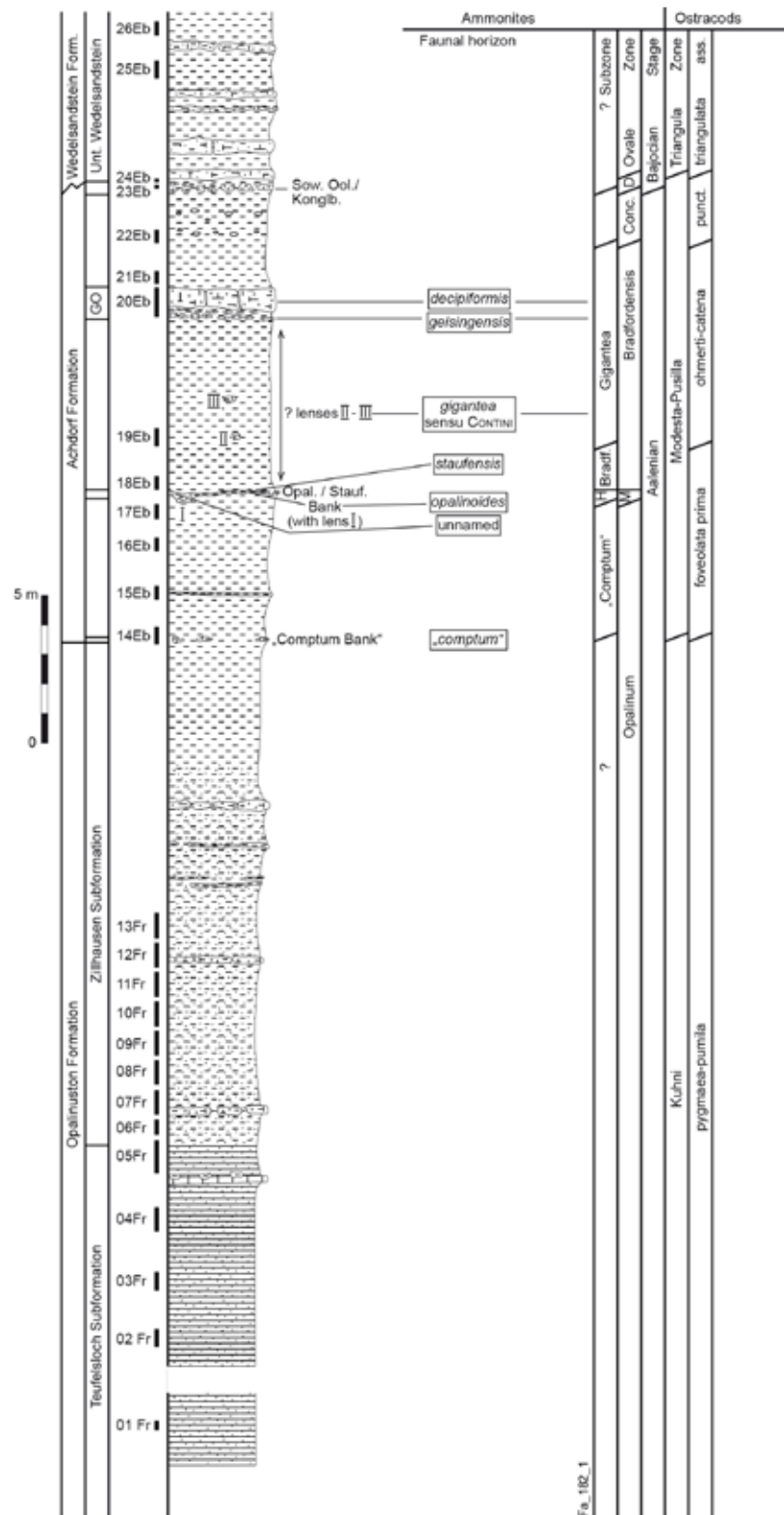
Fig. 2. Section of the Aalenian and Lower Bajocian in the Geisingen clay pit with correlation of the ammonite biostratigraphy and the ostracod faunal assemblages. Abbreviations: GO = Geisingen Oolite, Sow. Ool. = Sowerbyi Oolite, Kongl.b. = Konglomeratbank, Opal. / Stauf. Bank = Opalinoides /Staufensis Bank, H = Haugi, Bradf. = Bradfordensis, M = Murchisonae, Conc. = Concavum, D = Discites, punct. = punctulata, ass. = assemblage. Diagonal lines: boundary not exactly known.
