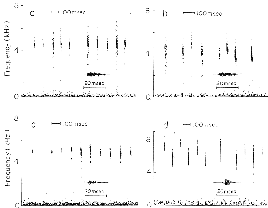
FIG. 1. Sonograms and oscillograms of regular pulses emitted by C. brachyotis (a), C. horsfieldi (b), M. ecaudatus (c) and M. sobrinus (d).
