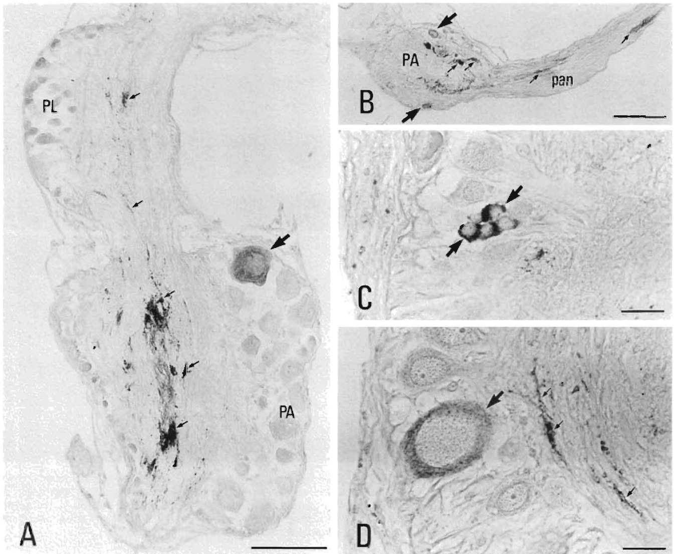
Fig. 3. Photomicrographs showing Gal-IR cells and fibers in the left pleural, parietal (A,B), and pedal (C, D) ganglia. A: Gal-IR fibers (small arrows) in the neuropil of the pleural (PL) and parietal (PA) ganglia and one large Gal-IR cell (large arrow). B: Two medium Gal-IR cells (large arrows) in the parietal ganglion (PA) and immunoreactive fiber bundles (small arrows) in the neuropil of the ganglion and the pallial nerve (pan). In these two planes, no small Gal-IR cells are seen. C: Small Gal-IR cells (arrows) in the pedal ganglion. D: One large Gal-IR cell (large arrow) in the pedal ganglion and immunoreactive fibers (small arrows) in the centrally located neuropil. Scale bars: A, B, 100 µm; C, D, 20 µm.
