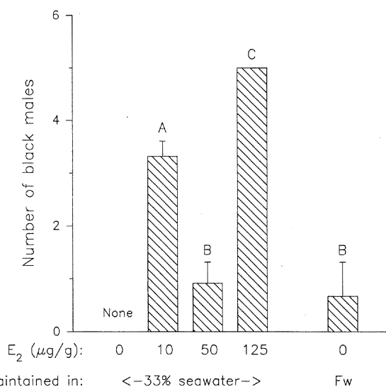
Fig. 4. Numbers of black males (mean ± S.E.) observed daily on days 7 - 9 after groups of 15 males were implanted with different dosages of E 2 and maintained in 33% seawater (experiment 2): an additional control group was transferred back to freshwater on the day after the implant operation. Groups with the same letter are not significantly different from each other ( P > 0.05 , Mann-Whitney U test).
