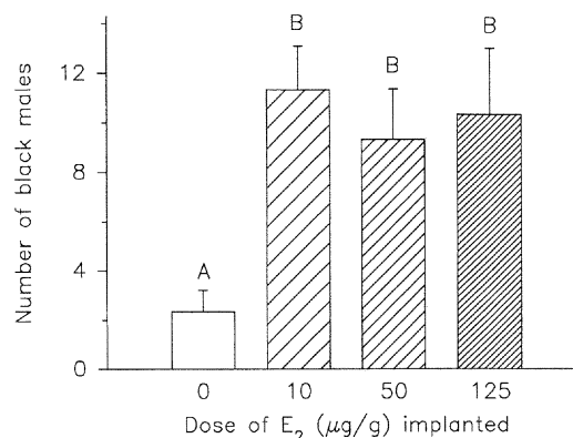
Fig. 5. (top) Daily fluctuations in the numbers of black males in groups of 15 males implanted with different dosages of E 2 : all groups were transferred back to freshwater on the day after the implant operation (experiment 3). (bottom) Numbers of black males (mean ± S.E.) observed daily on days 7 - 9 for the same experiment. Groups with the same letter are not significantly different from each other ( P > 0.05 , Duncan's test).
