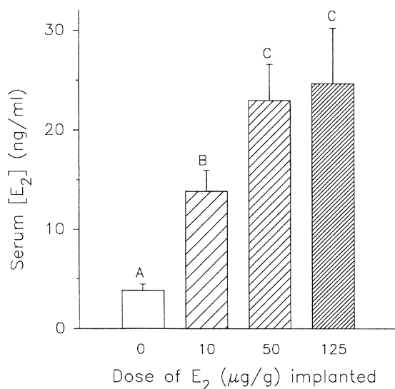
Fig. 1. The effects of different dosages of E_2 (0–125 \mu\text{g/g} ) on serum E_2 levels of males maintained in 33% seawater for 14 days (mean + S. E.; N = 6 for each): A, B and C are significantly different from each other ( P < 0.05 ).
