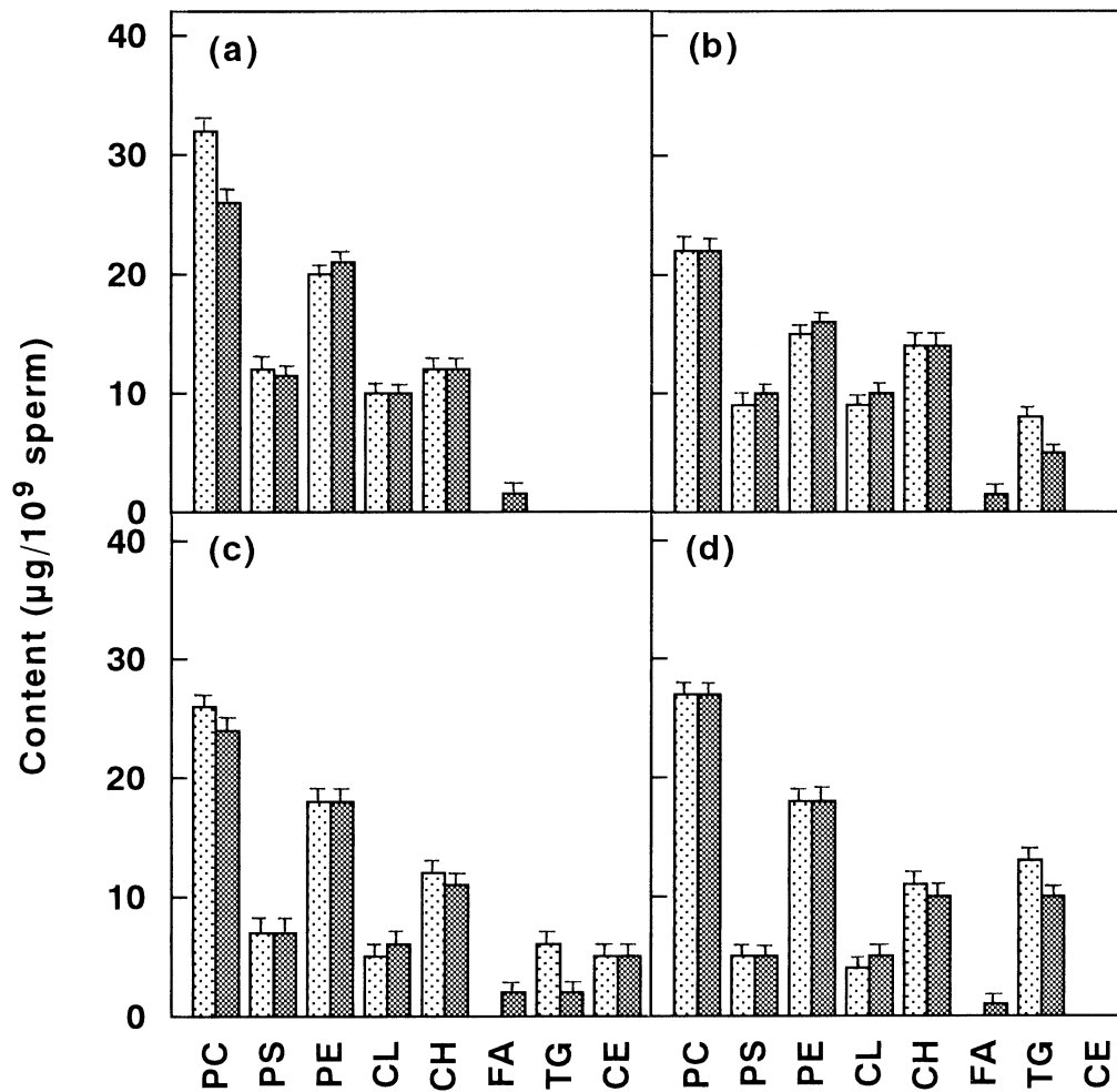
Fig. 3. Changes in lipid levels after incubation of spermatozoa of Hemicentrotus pulcherrimus (a), Glyptocidaris crenularis (b), Clypeaster japonicus (c) and Diadema setosum (d). Before (clear) and after (dotted) 100-fold dilution and incubation of dry sperm in seawater for 1 hr at 20°C, lipids were extracted and analyzed. Each value is the mean \pm SEM of four separate experiments. PC, phosphatidylcholine; PS, phosphatidylserine; PE, phosphatidylethanolamine; CL, cardiolipin; CH, cholesterol; FA, fatty acid; TG, triglyceride; CE, cholesterol-ester.
