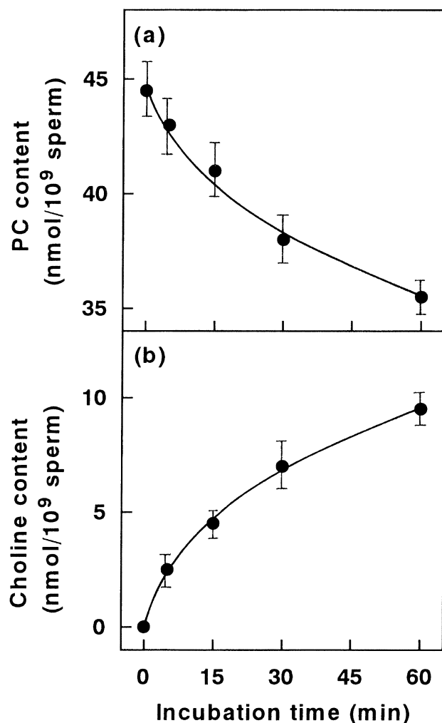
Fig. 4. Changes in levels of phosphatidylcholine (a) and choline (b) following incubation of Hemicentrotus pulcherrimus spermatozoa in seawater. Each value is the mean \pm SEM of four separate experiments.
