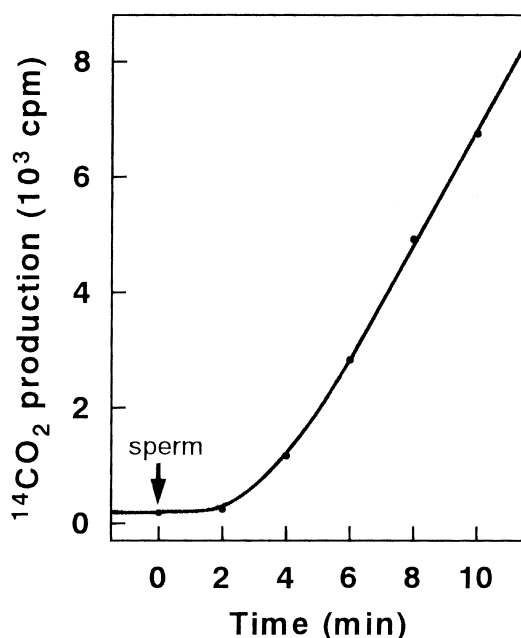
Fig. 2. Oxidation of fatty acid in Hemicentrotus pulcherrimus spermatozoa. Dry sperm were diluted 100-fold in seawater containing [1- 14 C]oleic acid and carbonic anhydrase in a total volume of 10 ml at 20°C. Radioactivity in the 14 CO 2 produced was counted by the thin-window gas flow counter.
