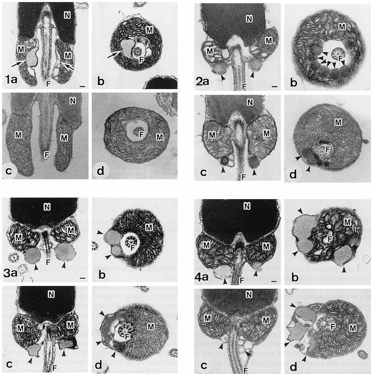
Fig. 7. Longitudinal (a,c) and transverse (b,d) sections through the mitochondrial region of Hemicentrotus pulcherrimus (1), Glyptocidaris crenularis (2), Clypeaster japonicus (3) and Diadema setosum (4) spermatozoa before (a,b) and after incubation in seawater for 30 min (c,d). Arrows and arrow heads show lipid bodies and lipid globules, respectively. F, flagellum; M, mitochondrion; N, nucleus. Bars show 0.1 \mu\text{m} .
