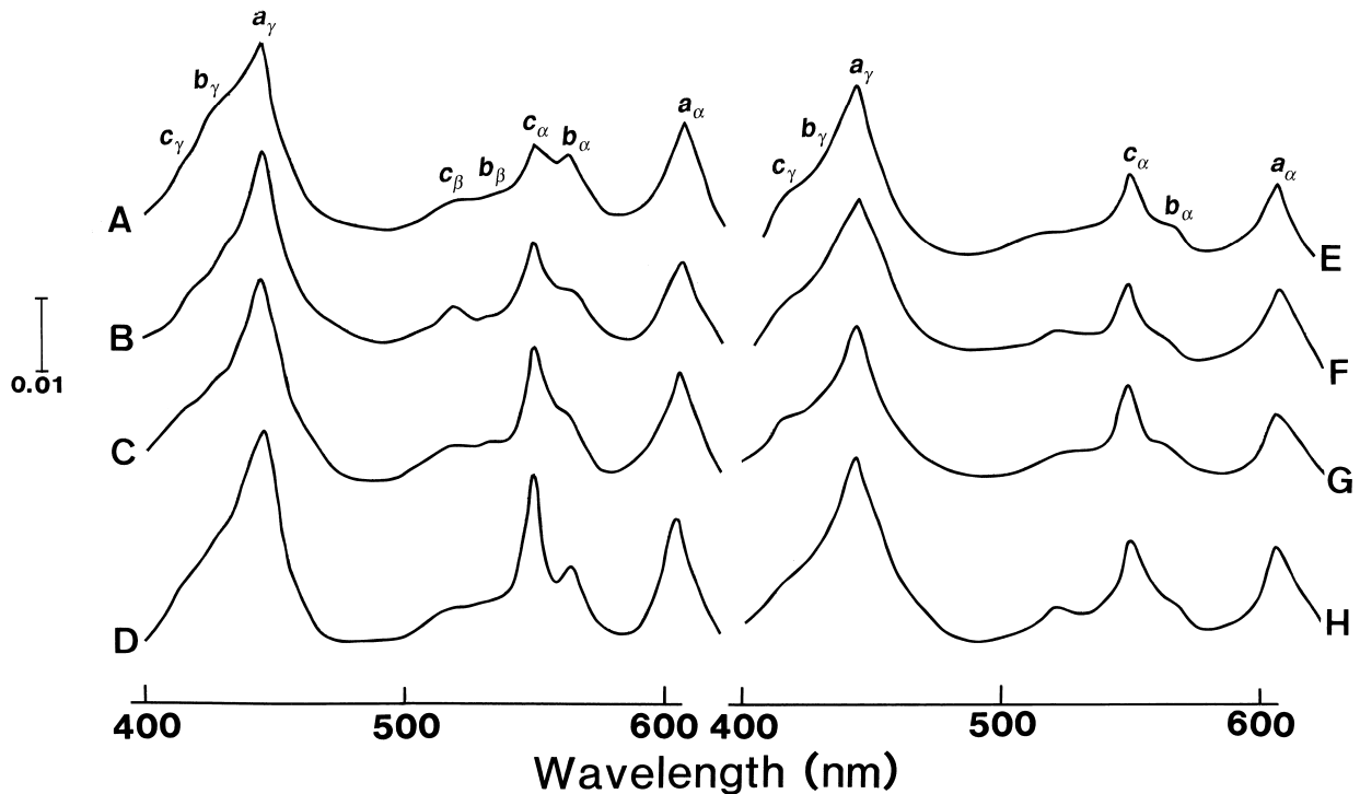
Fig. 4. Difference spectra between hydrosulfite-reduced and \text{H}_2\text{O}_2 -oxidized mitochondrial suspensions isolated from sperm of echiuroid, sea urchin, oyster and tunicate. Difference spectra were obtained on suspensions containing 10^{10} cell equivalent/ml of mitochondria, isolated from sperm of echiuroid (A, E), sea urchin (B, F), oyster (C, G) and tunicate (D, H). Mitochondria were isolated from fresh sperm (A–D) and sperm incubated for 15 hr at 20^\circ\text{C} (E–H). Recovery of mitochondria, judged on the basis of cytochrome c oxidase, was at least 86.6%. Peaks of cytochromes are specified with a_\alpha , a_\gamma for cytochrome aa_3 , b_\alpha , b_\beta , b_\gamma for cytochrome b and c_\alpha , c_\beta , c_\gamma for cytochrome c . Vertical bar shows 0.01 in absorbance.
